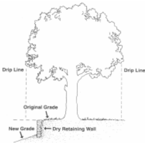
Figure 2. Construct a retaining wall when grade is lowered.
